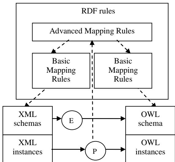
Fig. 2. Relations between processes and RDF rules.
