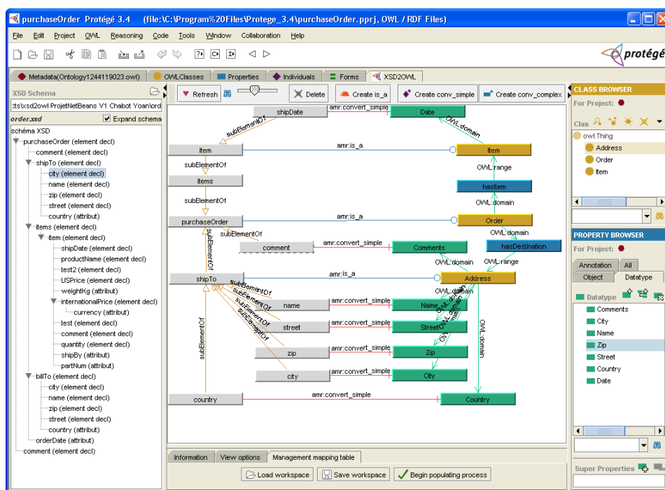
Fig. 1. Snapshot of the XSD2OWL plug-in.
